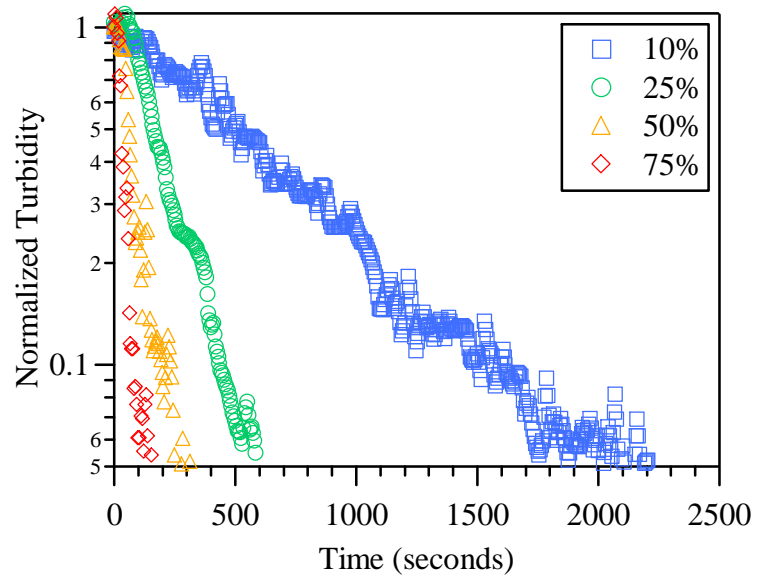
Figure 3.1: Settling of composites at various weight percentage of titania in each particle
