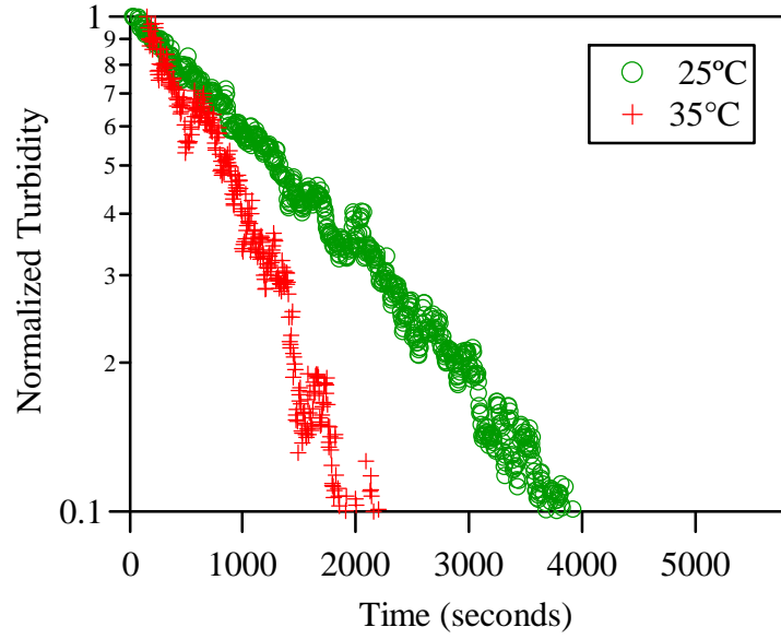
Figure 4.4: Settling of composite with 25% ceria at temperatures below and above the transition temperature ( T \sim 32^\circ\text{C} )
