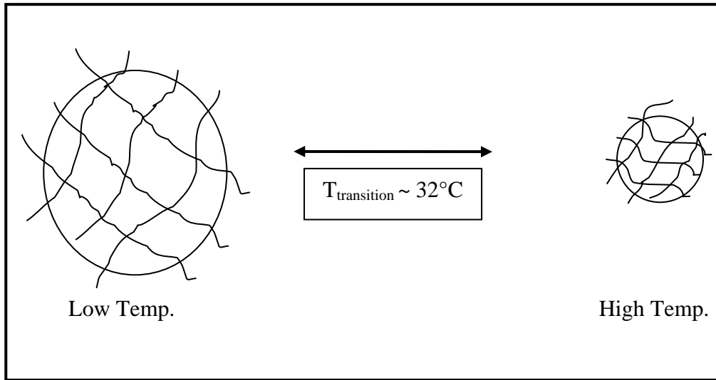
Figure 3.2 Schematic of microgel response above and below the volume phase transition temperature.
