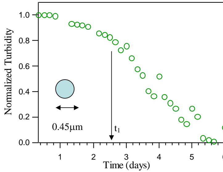
Figure 2.5 Normalized turbidity signal for the settling 'fine' silica sphere
