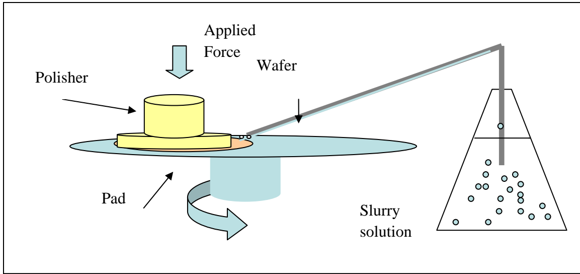
Figure 4.1 Schematic of slurry polishing in a CMP process.
