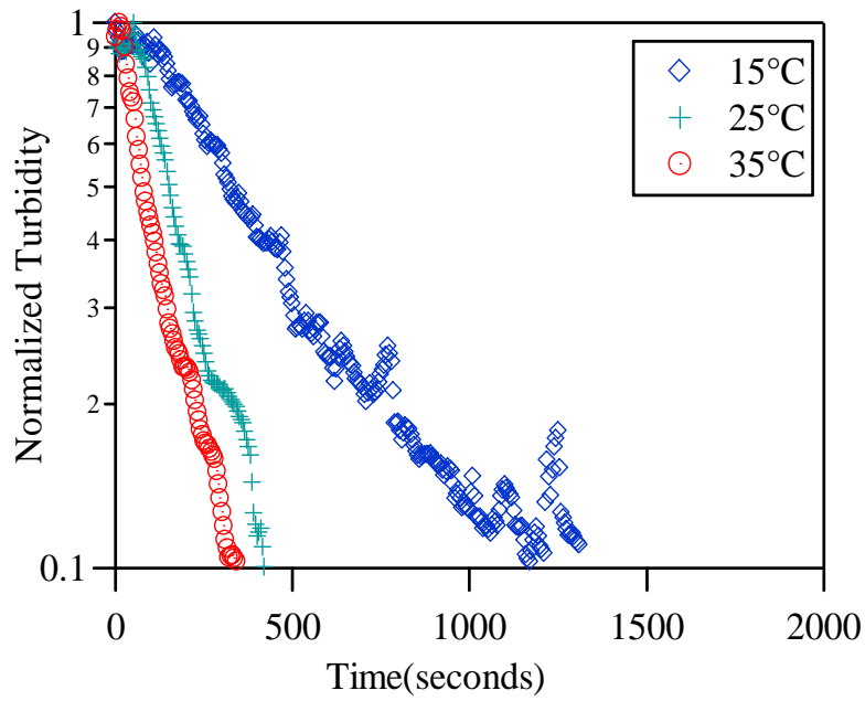
Figure 3.3 Settling of composite with 25% titania at temperatures below and above transition temperature ( T \sim 32^\circ\text{C} )
