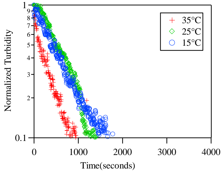
Figure 4.3: Settling of composite with 50% ceria at temperatures below and above the transition temperature ( T \sim 32^\circ\text{C} )
