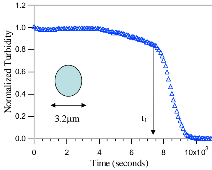
Figure 2.4 Normalized turbidity signal for the settling 'large' silica spheres
