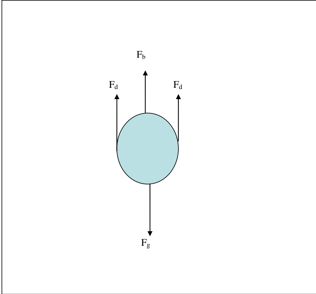
Figure 2.2 Schematic of forces acting on a particle settling in liquid
