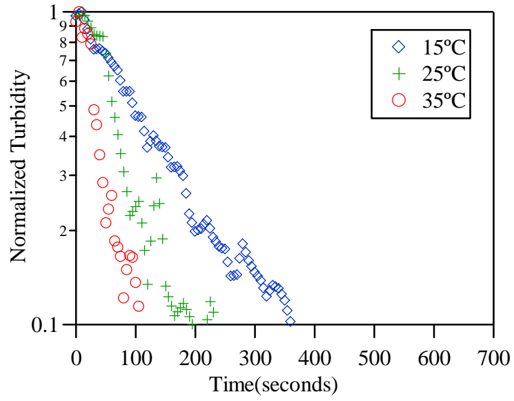
Figure 3.4 Settling of composite with 50% titania at temperatures below and above transition temperature ( T \sim 32^\circ\text{C} )
