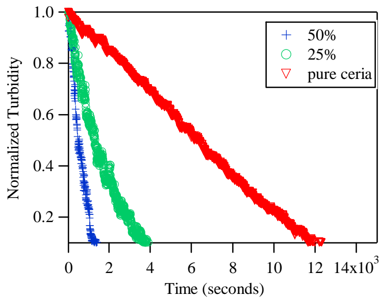
Figure 4.2 Settling of pure ceria nanoparticles at ambient temperature compared against composites with 25% and 50% ceria loading.
